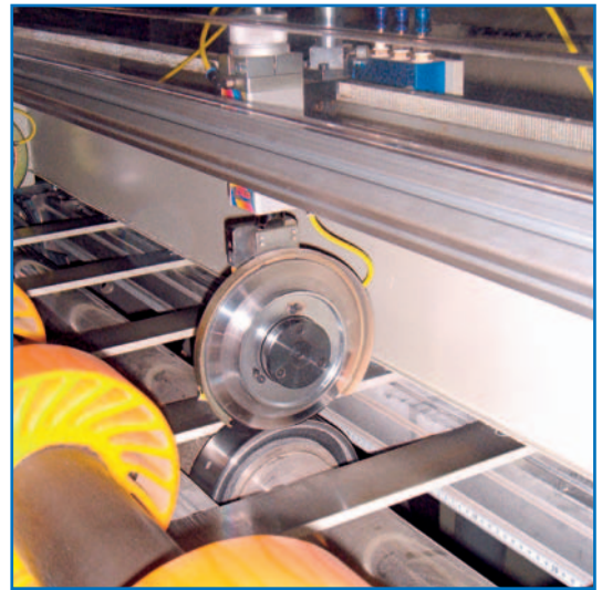
Slitting knife (pneumatic knife holder)
