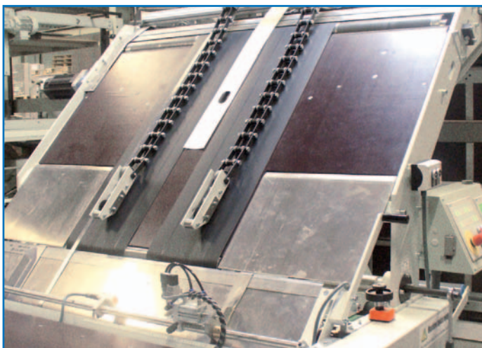
Automatic Laminator
